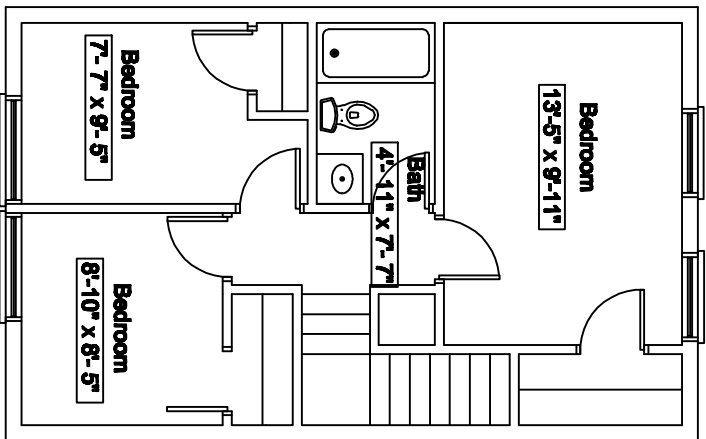
Marconi Townhouse- 2nd Floor
