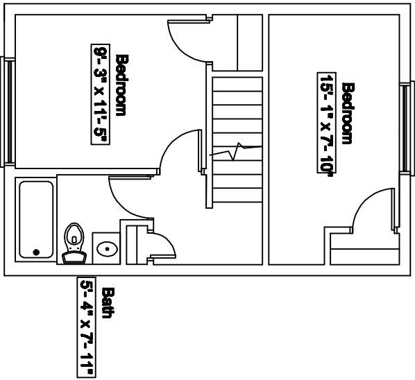
Limberlost 2 Bedroom- 2nd Floor
